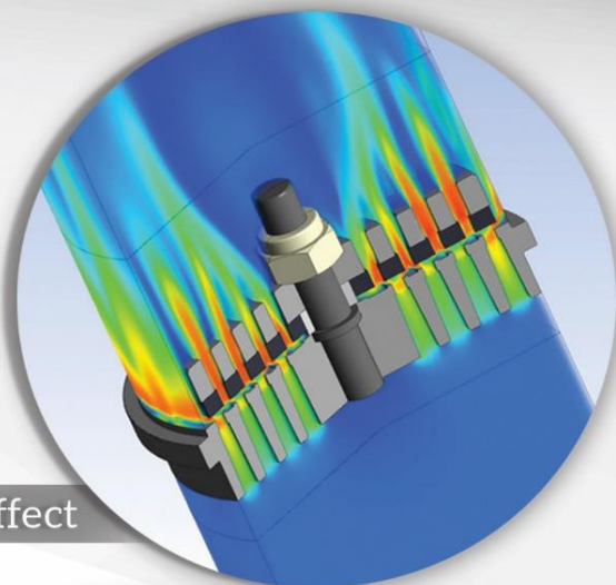
Stone Trap Design
